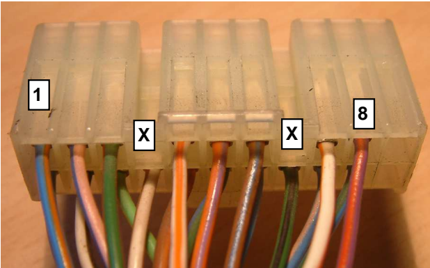
Flat plug new (no Clip)
